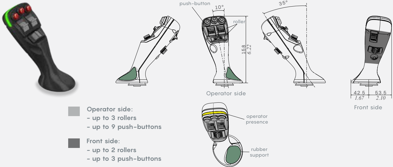
Standard push-buttons configuration
